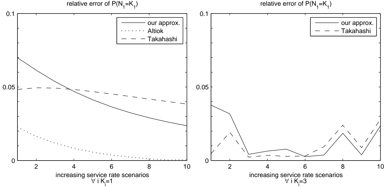
Figure 2: Comparison with the methods of Altiok and Perros (1987) and of Takahashi, Miyahara and Hasegawa (1980) under two capacity configurations.
